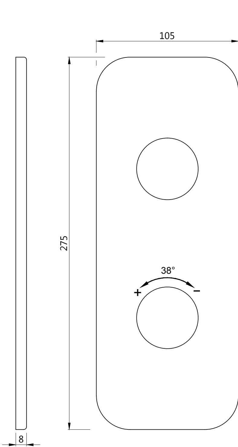
WALL FLANGE
